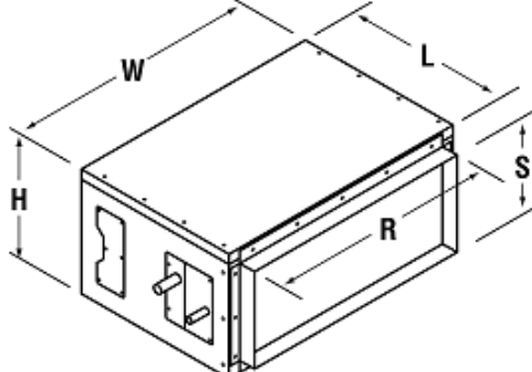
Figure 19: Coil Module Dimensions
