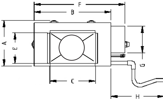
Figure 16: Outline Dimensions - Front View
