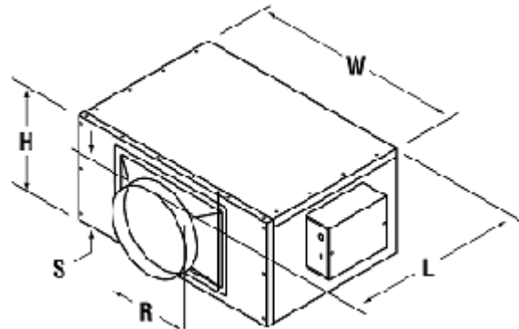
Figure 18: Blower Module Dimensions
