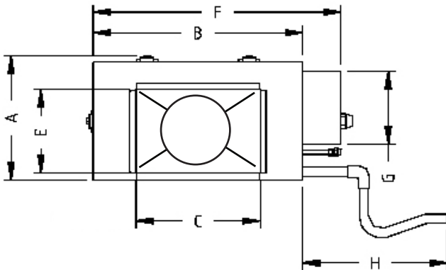
Figure 16: Outline Dimensions - Front View
